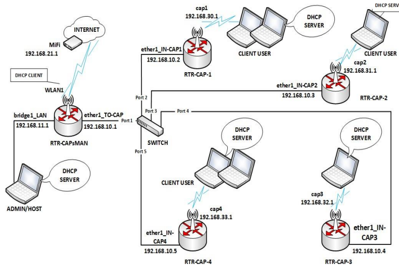
Figure 3 Logic Topology Design
